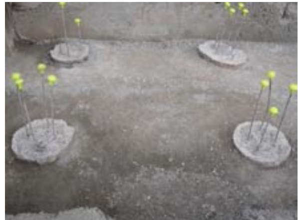
Good pile head preparation
