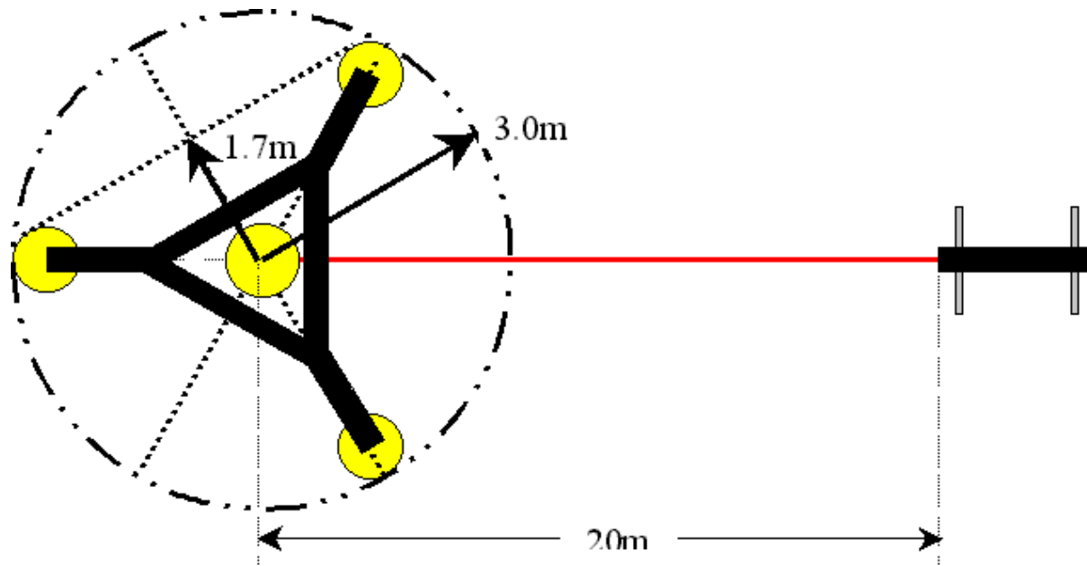
STATNOMIC Plan View
